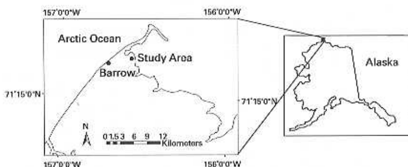
Figure 1 Study area location near Barrow, Alaska
