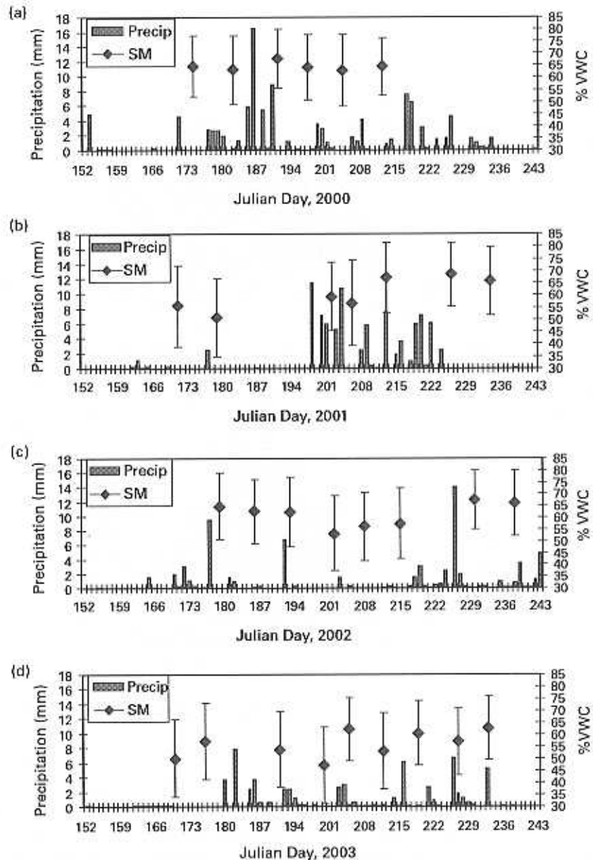
Figure 4 Daily precipitation and average near surface soil moisture for each measurement day plotted over time for a) 2000, b) 2001, c) 2002 and d) 2003. Error bars on the surface soil moisture points represent plus and minus one standard deviation
