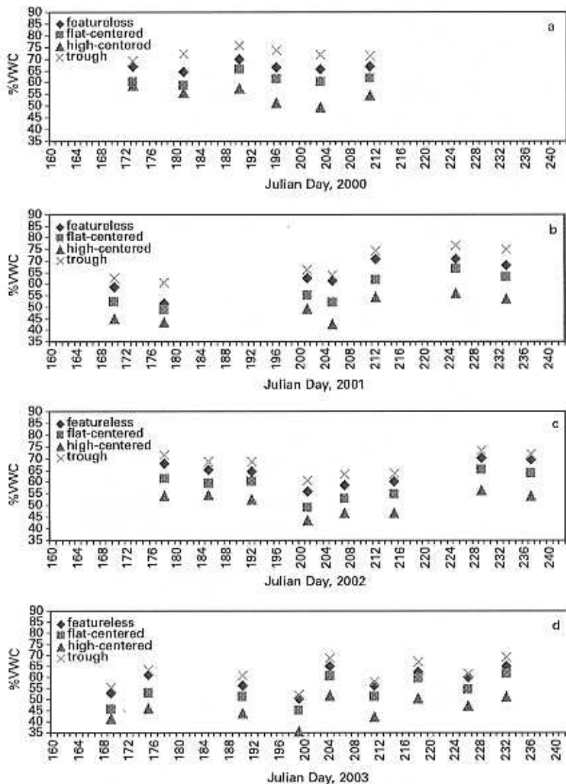
Figure 5 Average near surface soil moisture at the four microsite types in (a) 2000, (b) 2001, (c) 2002 and (d) 2003
